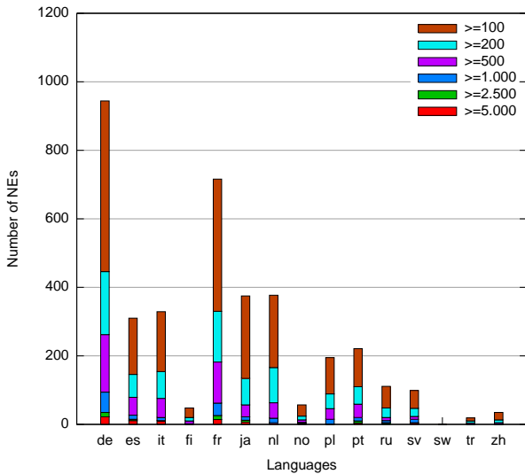
Number of NEs dependent on context number - ambiguous dataset
