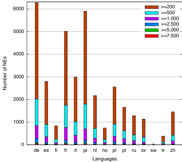
Number of NEs dependent on context number - complete dataset
